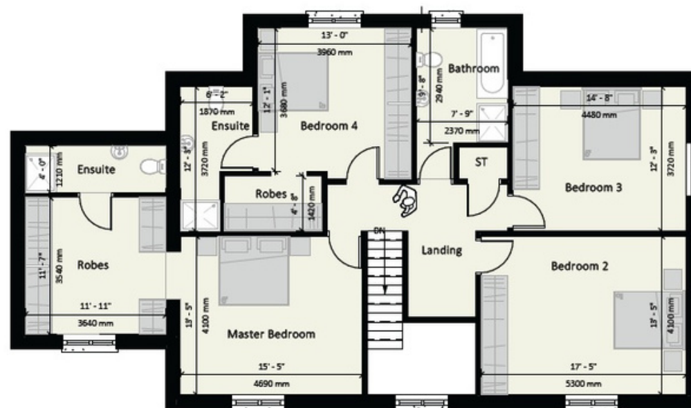
First Floor
