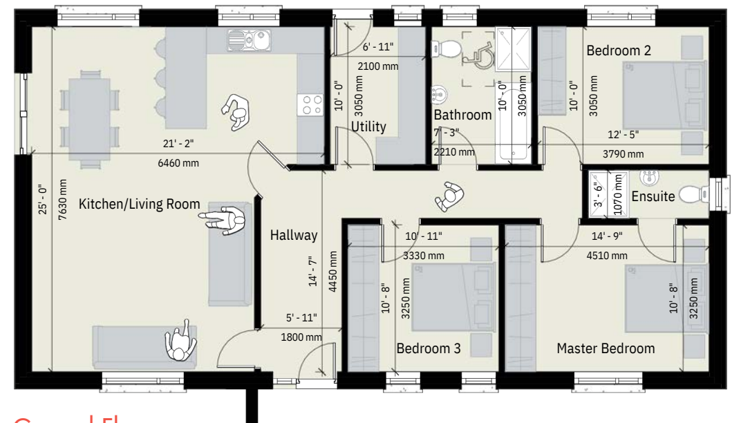
Ground Floor
