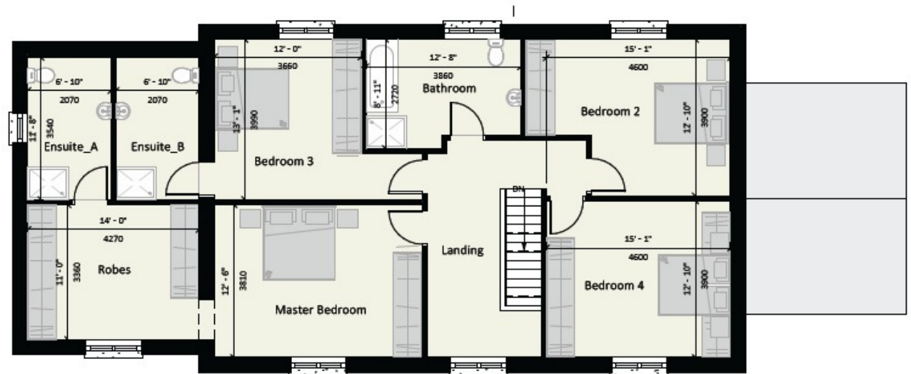
First Floor
