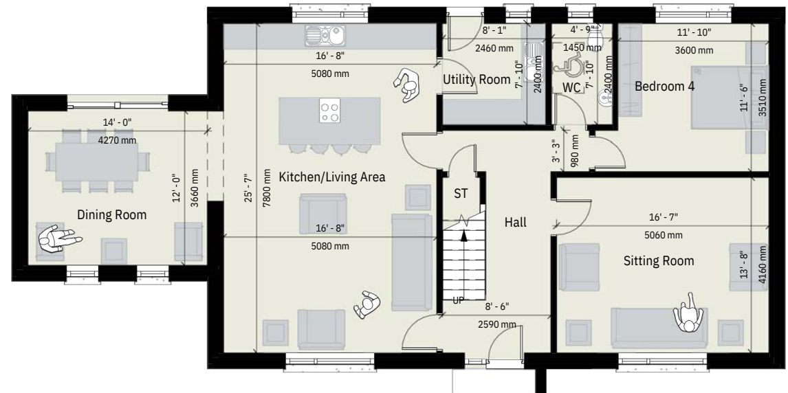
Ground Floor
